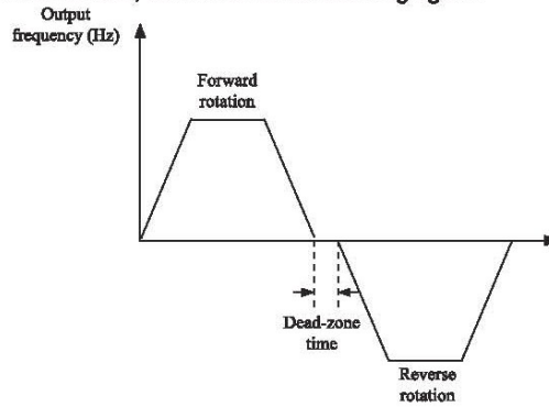
Figure 4-13 Forward/Reverse rotation dead-zone time
