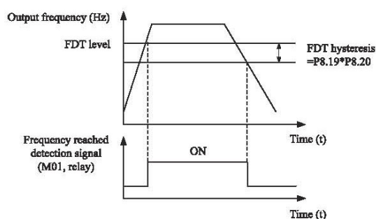
Figure 4-14 FDT level
